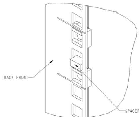
Figure 2-5. Installing the Tinnerman Nuts and Spacers (Compaq/Rittal Rack)
